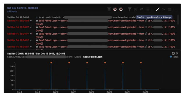
Figure 31: A graph illustrating the repeated login attempts
