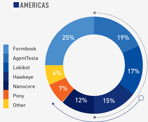
Figure 25: Top Infostealer Malware in the Americas
